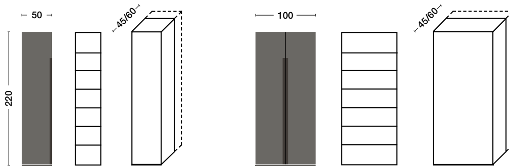
Schrank 220 Cabinet 220
